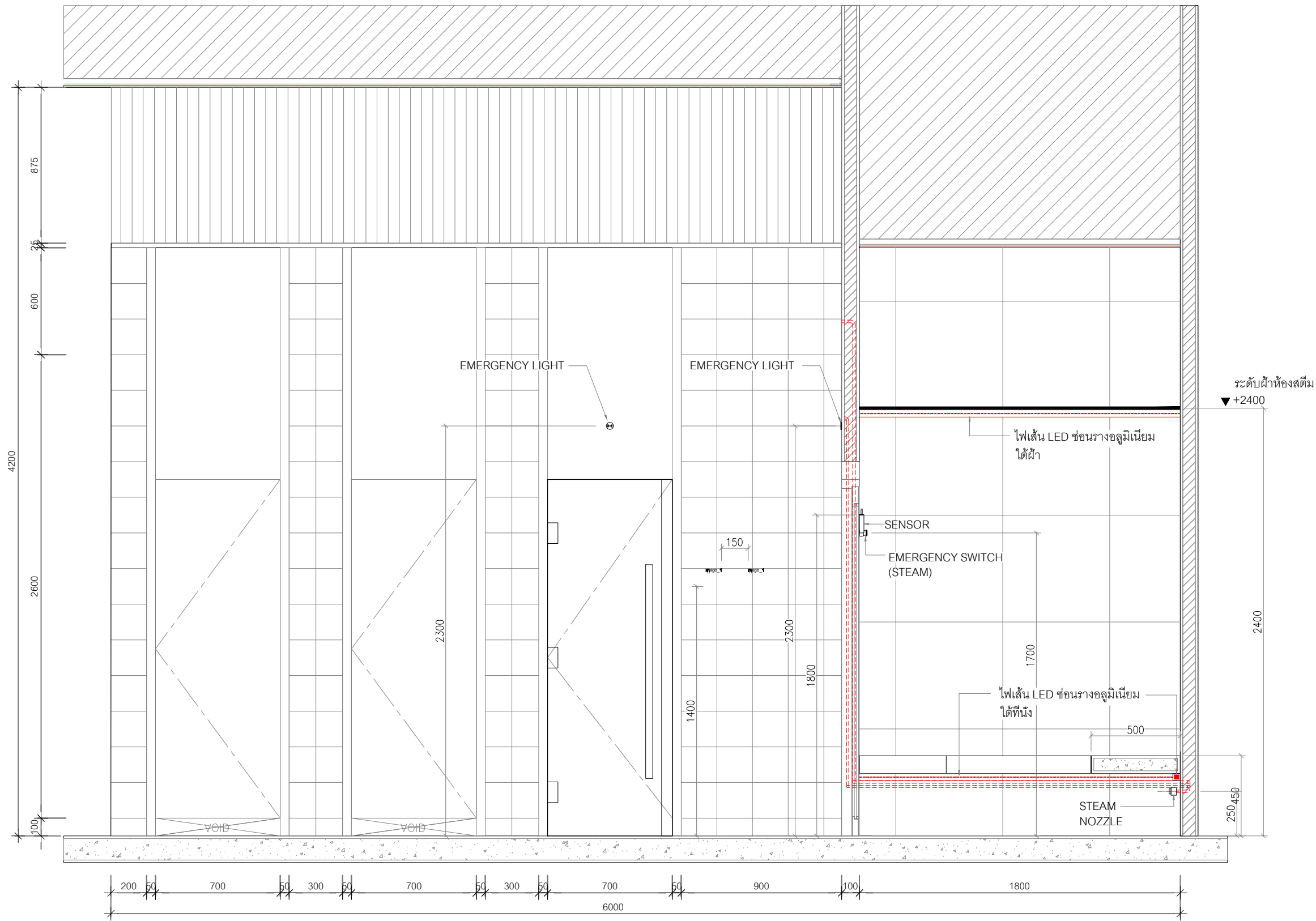
CLUB HOUSE ELEVATION SCALE 1 : 25
