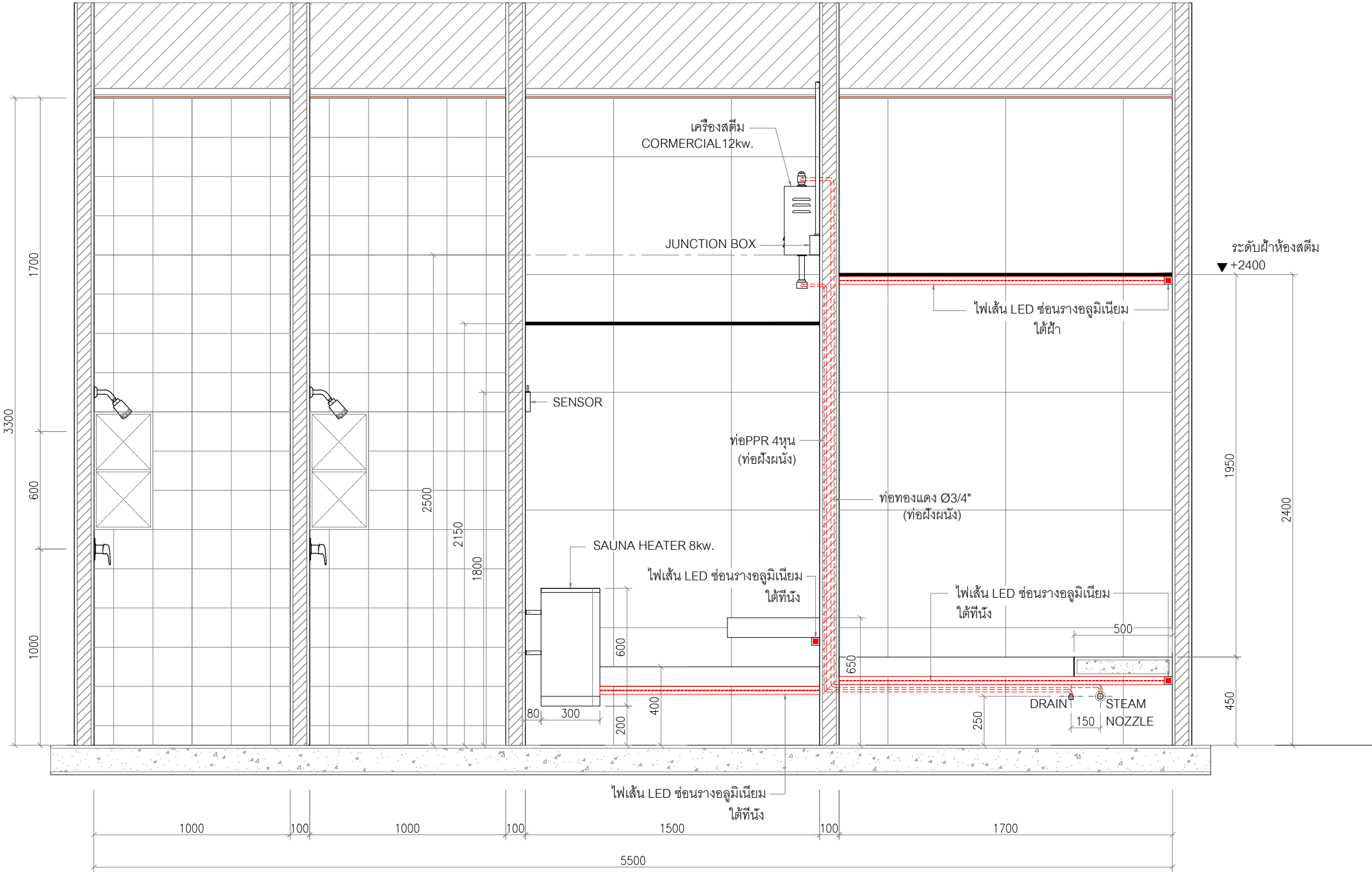
CLUB HOUSE ELEVATION SCALE 1 : 25
