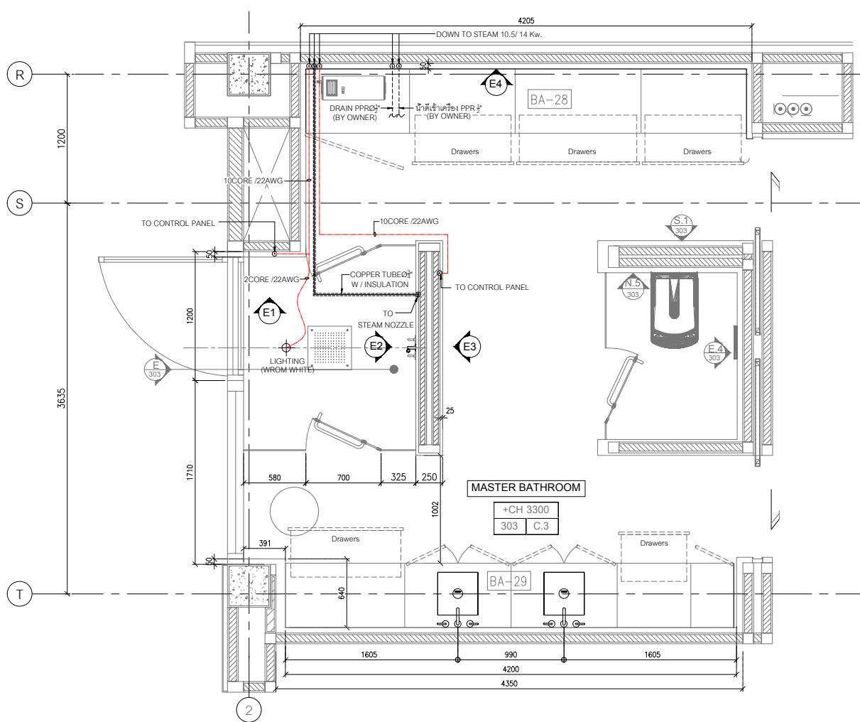
MASTER BATHROOM CEILING PLAN SCALE 1:50
