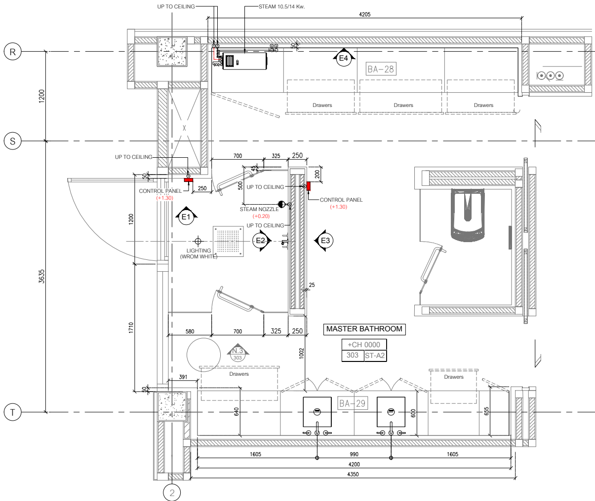
MASTER BATHROOM FLOOR PLAN SCALE 1:50
