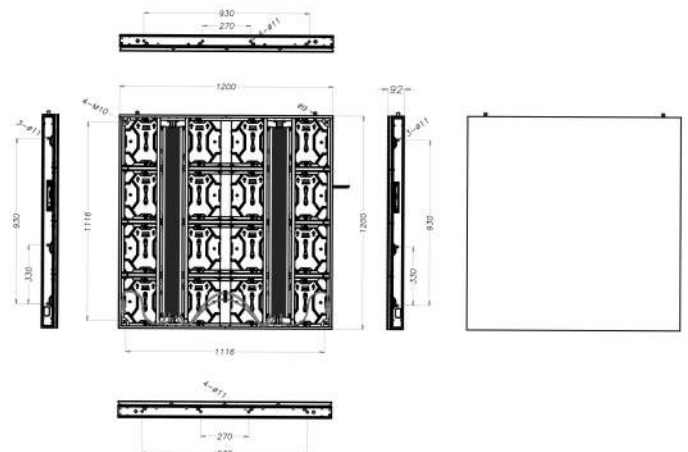
Cabinet drawing
