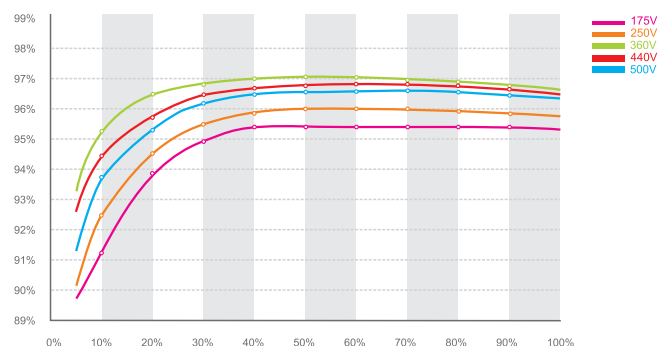
Growatt 6000MTL-10 efficiency
