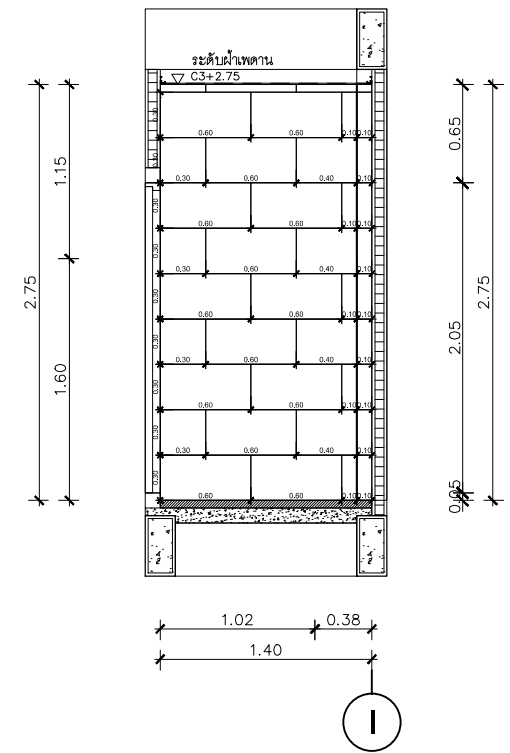
SECTION A SCALE 1:50
