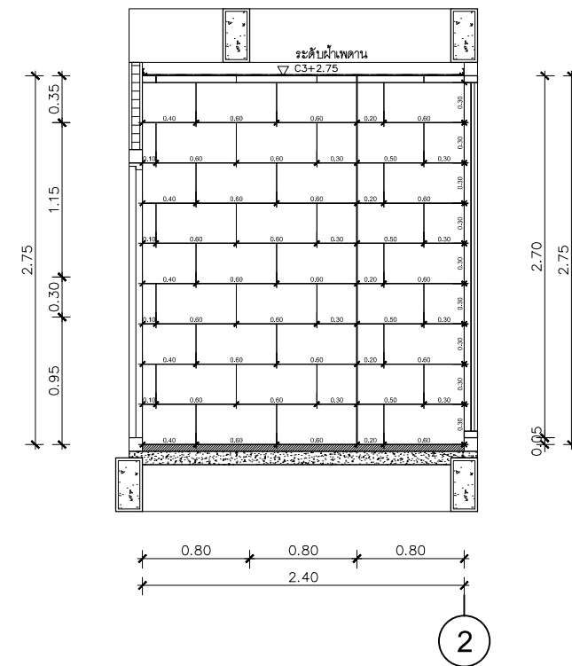
SECTION D SCALE 1:50
