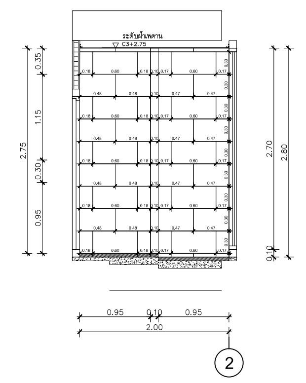
SECTION D SCALE 1:50
