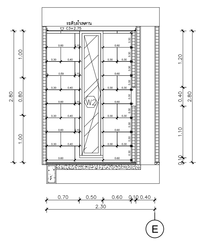
SECTION A SCALE 1:50
