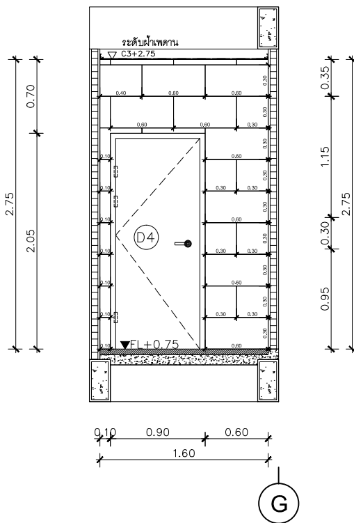
SECTION C SCALE 1:50
