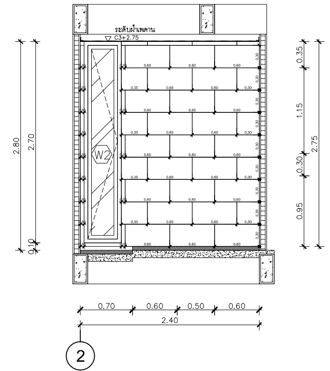
SECTION B SCALE 1:50
