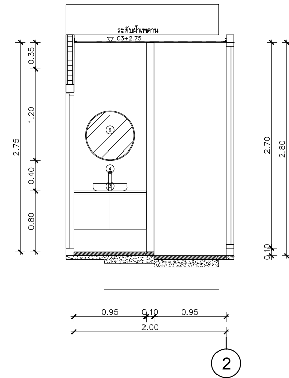
SECTION D SCALE 1:50
