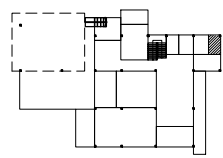
BATHROOM 2 ± FLOOR 1 SCALE 1:50
