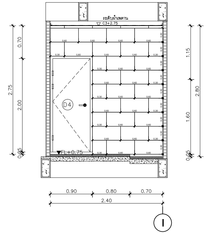
SECTION D SCALE 1:50
