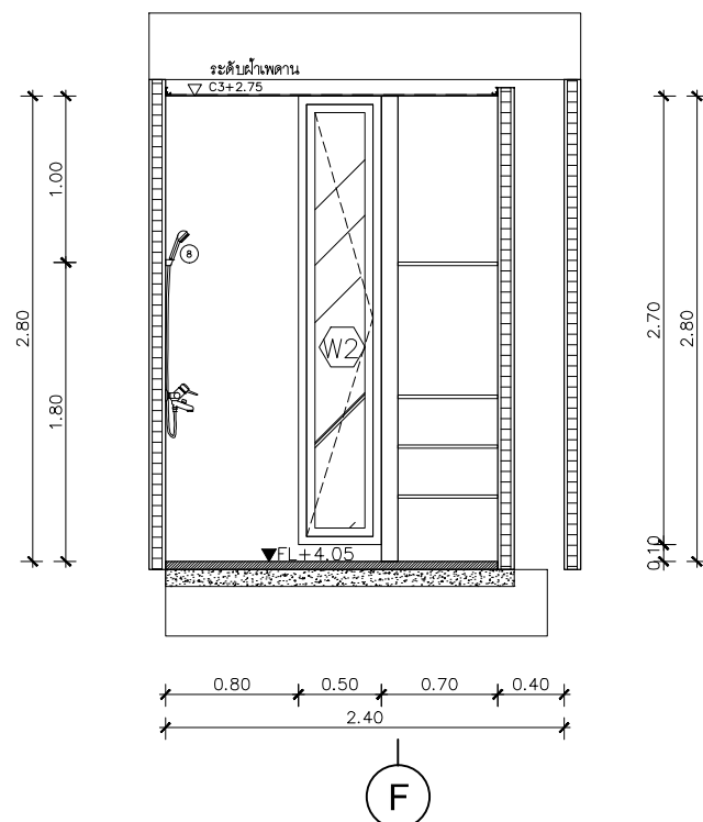
SECTION C SCALE 1:50
