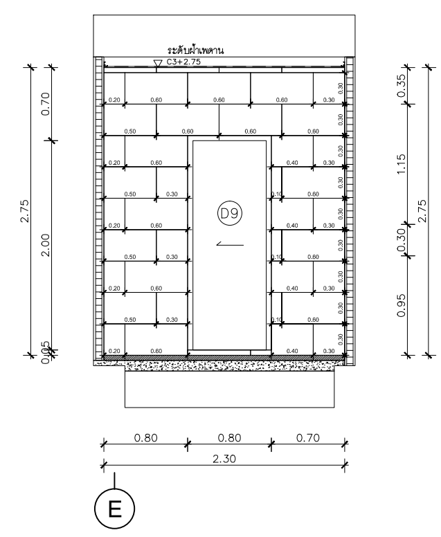
SECTION C SCALE 1:50
