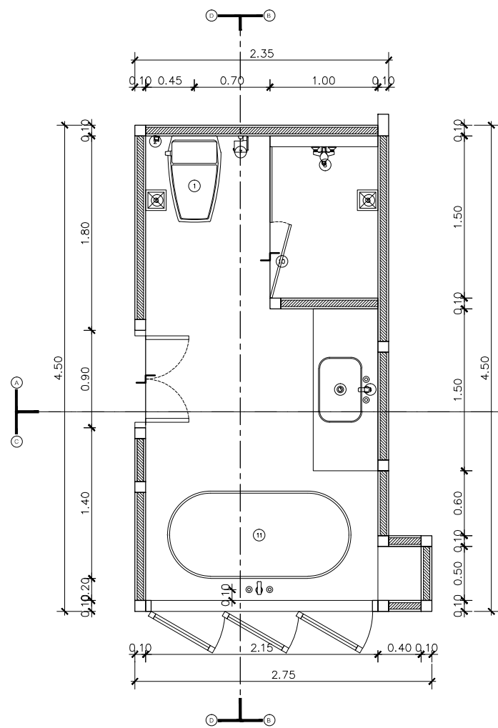
BATHROOM 6 (CHEE) ± FLOOR 2
