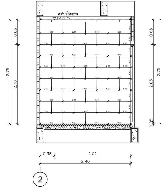
SECTION B SCALE 1:50
