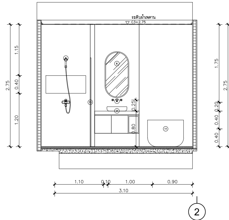
SECTION D SCALE 1:50
