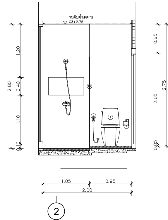
SECTION B SCALE 1:50
