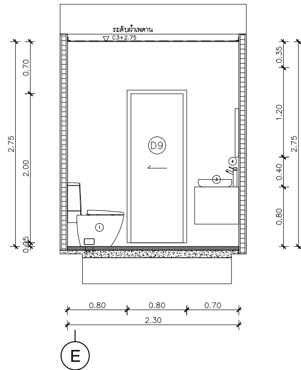
SECTION C SCALE 1:50
