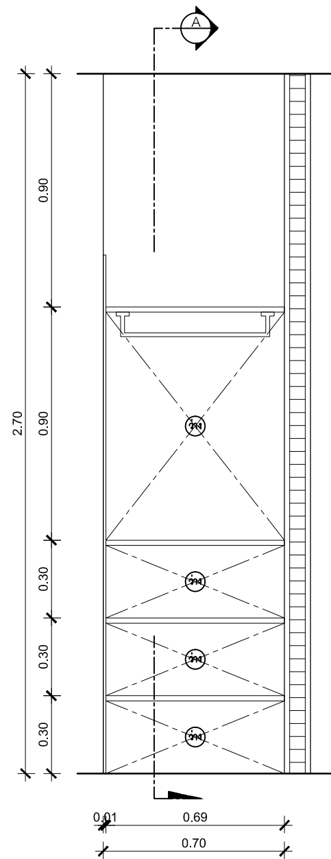
B4-07 ELEVATION SCALE 1:20
