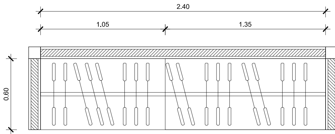
B4-04 PLAN SCALE 1: 20
