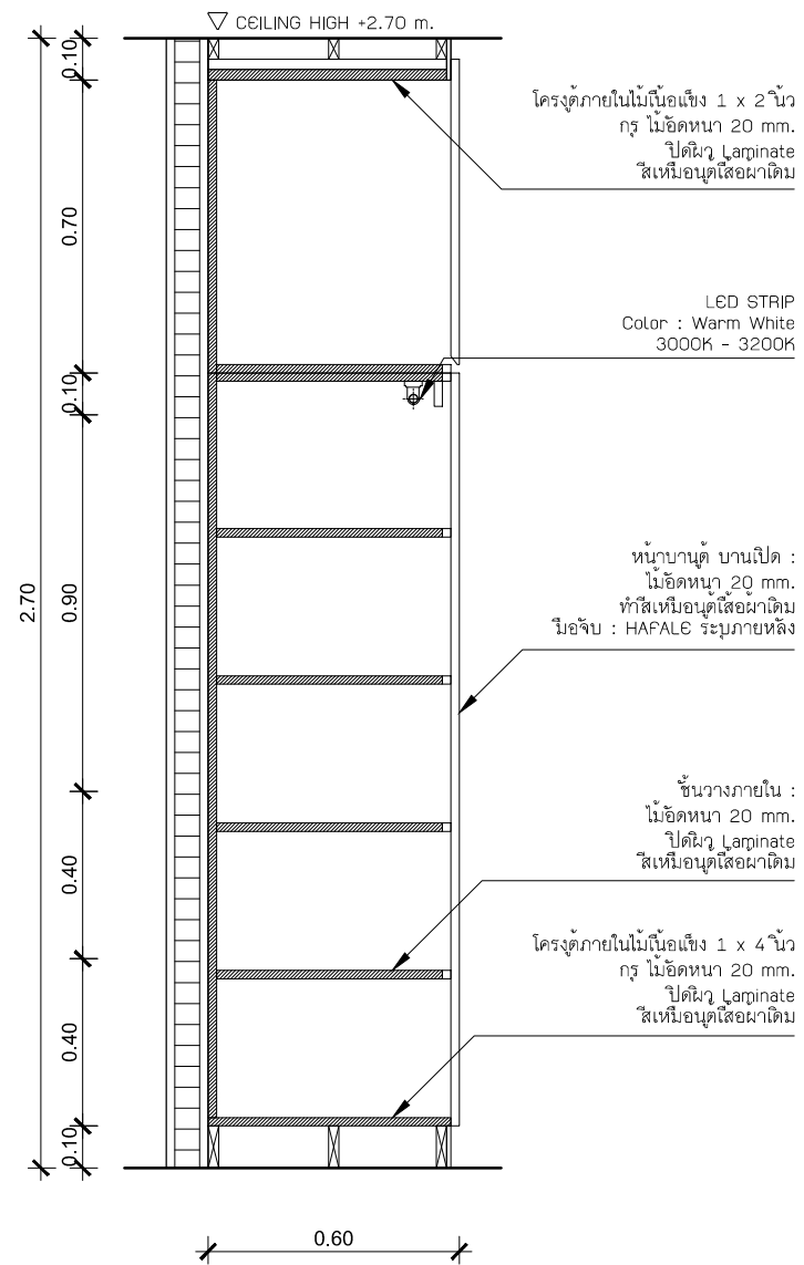
B4-04 SECTION A SCALE 1:20
