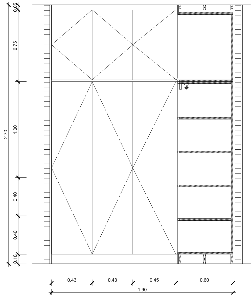
B4-04 ELEVATION SCALE 1:20
