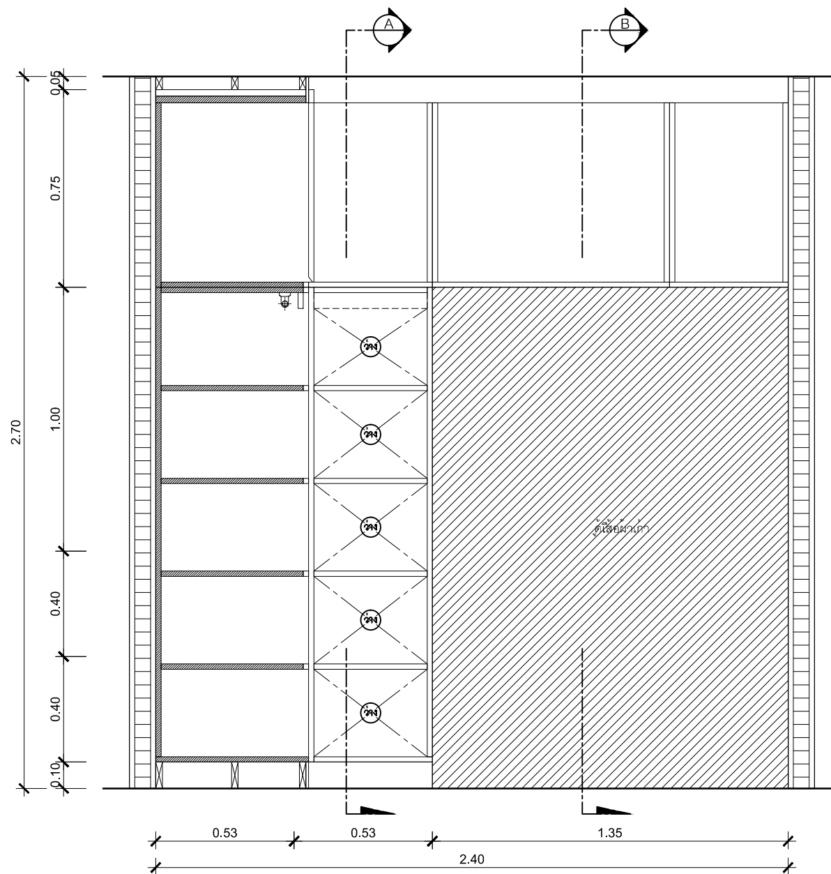
B4-04 ELEVATION (INSIDE) SCALE 1: 20
