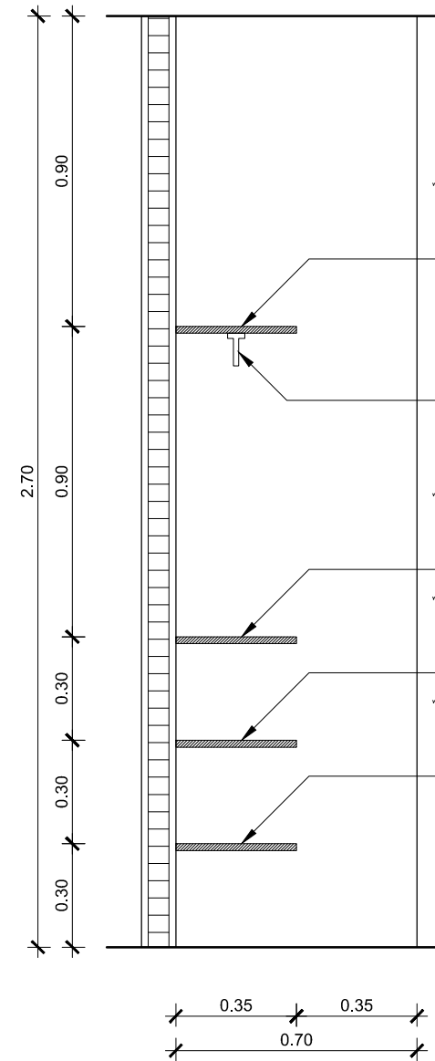
B4-07 SECTION A SCALE 1:20
