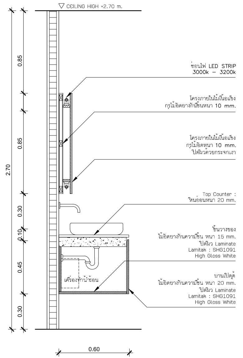
B4-06 SECTION A SCALE 1:20
