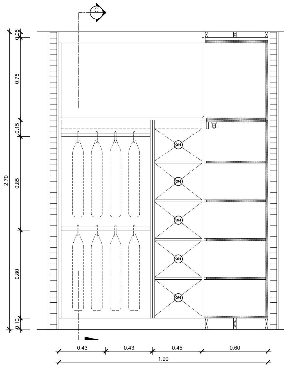
B4-04 ELEVATION (INSIDE) SCALE 1:20
