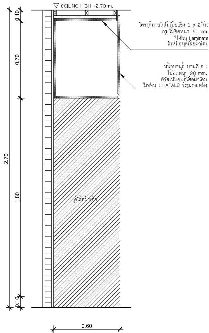
B4-04 SECTION B SCALE 1:20
