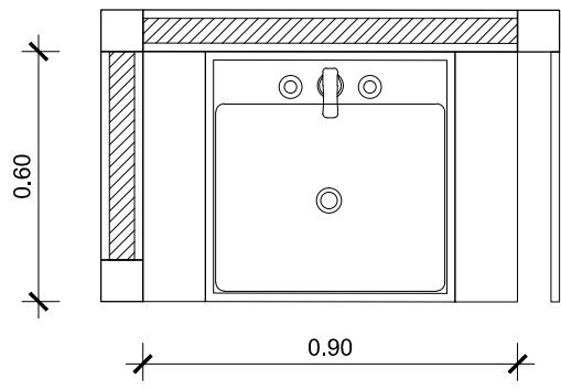
B4-06 PLAN SCALE 1:20
