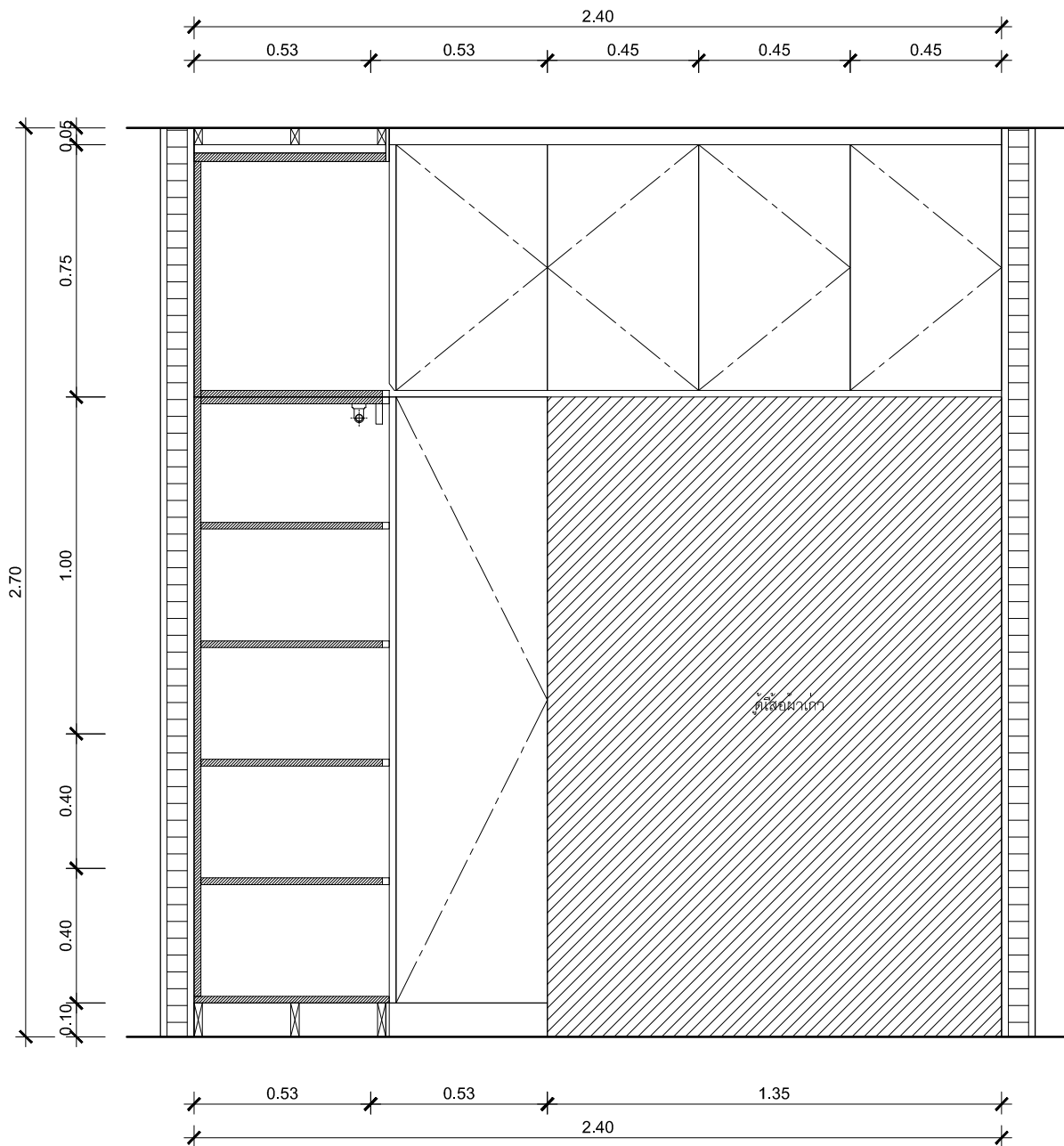
B4-04 ELEVATION SCALE 1: 20
