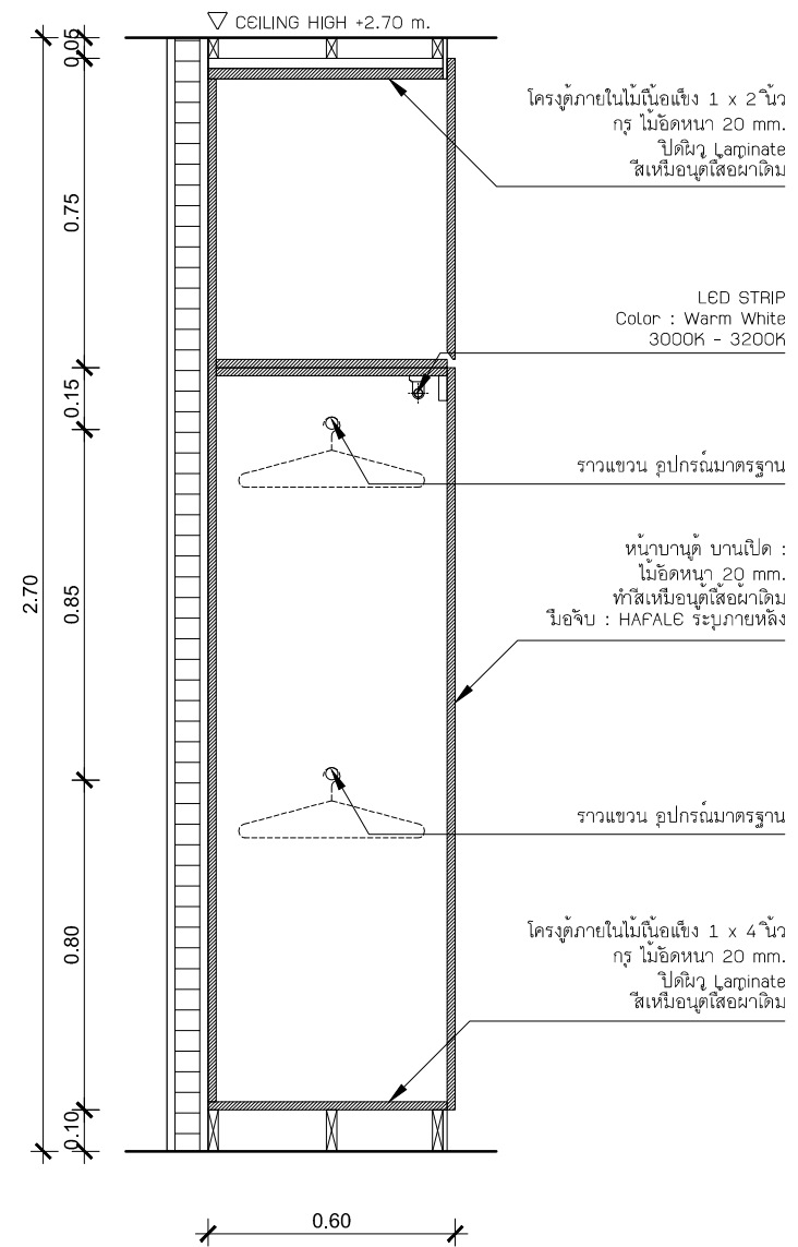
B4-04 SECTION C SCALE 1:20
