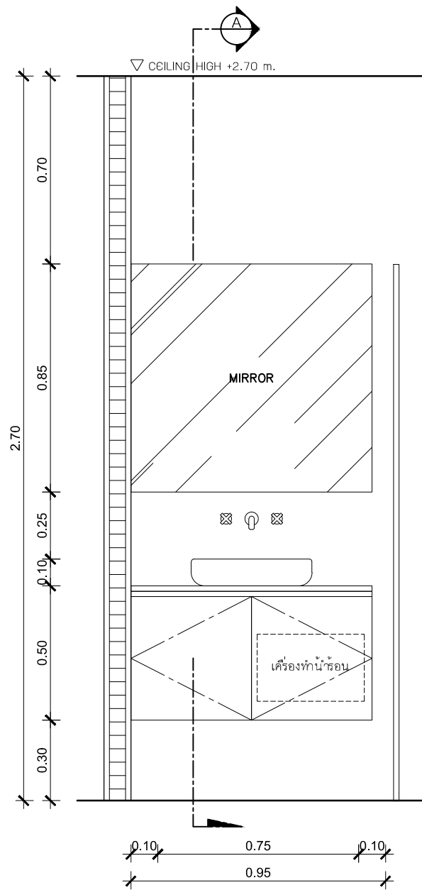
B4-06 ELEVATION SCALE 1:20
